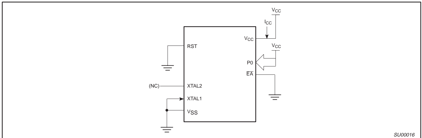
Figure 41. I_{CC} Test Condition, Power Down Mode All other pins are disconnected. V_{CC} = 2V to 5.5V
