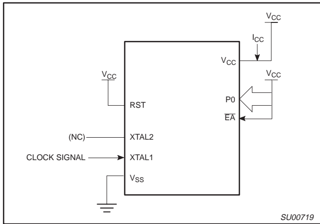
Figure 38. I_{CC} Test Condition, Active Mode All other pins are disconnected
