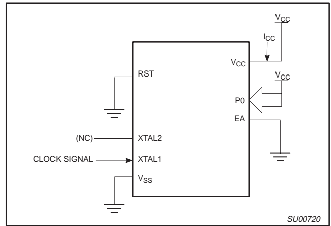
Figure 39. I_{CC} Test Condition, Idle Mode All other pins are disconnected
