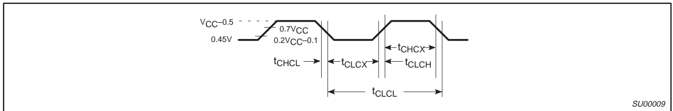
Figure 40. Clock Signal Waveform for I_{CC} Tests in Active and Idle Modes t_{CLCH} = t_{CHCL} = 5ns
