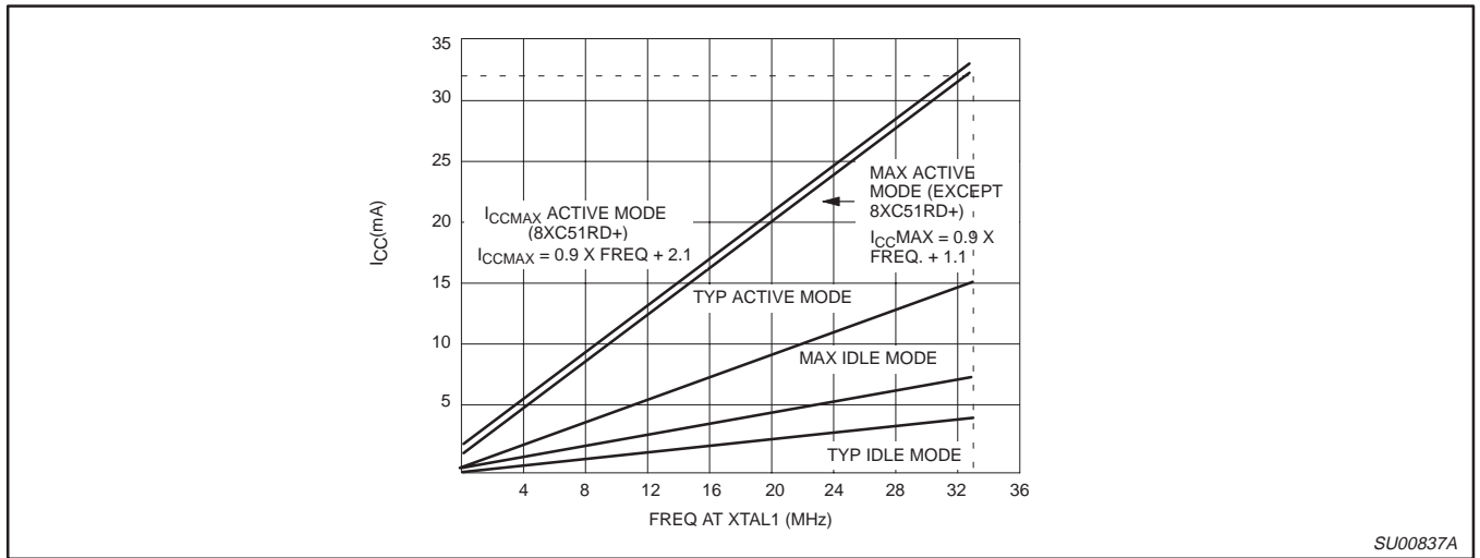
Figure 37. I_{CC} vs. FREQ Valid only within frequency specifications of the device under test
