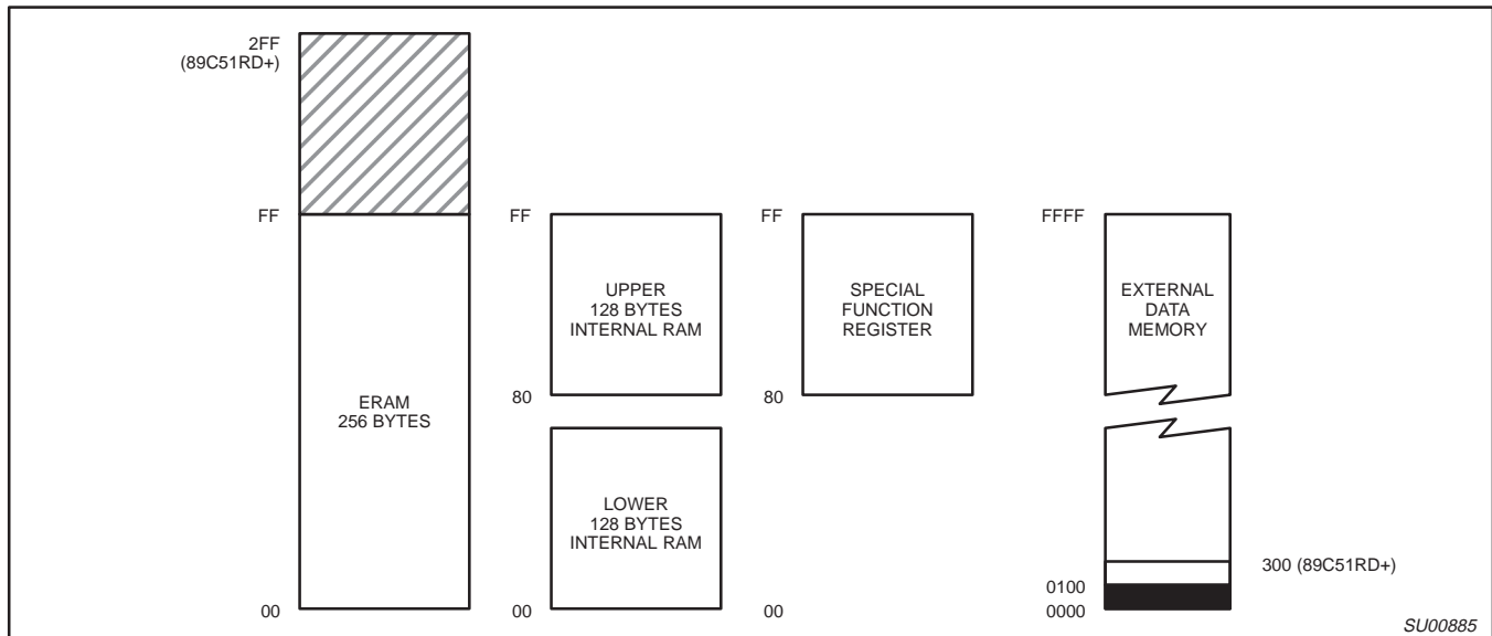
Figure 29. Internal and External Data Memory Address Space with EXTRAM = 0
